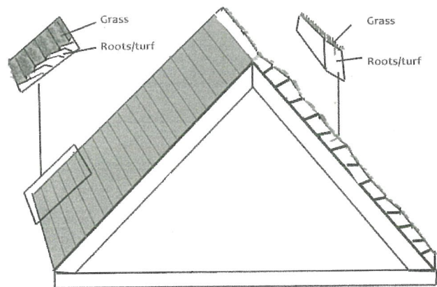
A turf-roof made of single-cut turf stringers
