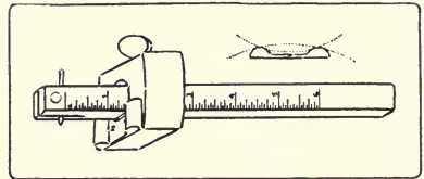
Fig. 215. Marking-Gage for Curves.
