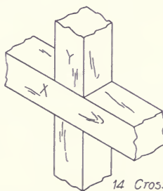
14 Cross-lap
