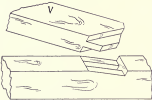
67 Oblique mortise-and-tenon
