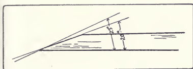
Fig. 78. Grinding Angle, 20^{\circ} ; Whetting Angle, 25^{\circ} .
