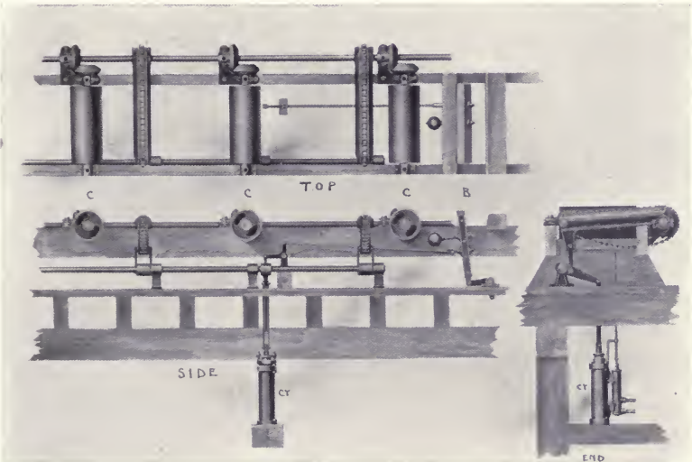
Fig. 44. Automatic Steam Transfer for Timber, Lumber and Slabs. The boards are carried along by the cylinders, C C C, until they hit the bumper, B. This movement admits steam to the cylinder, CY, which raises the revolving chains or skids, which transfers the stock sidewise to other live rollers as required.
