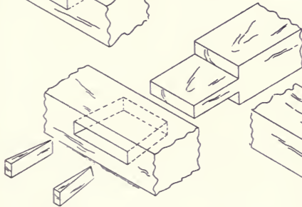
34 Wedged mortise-and-tenon
