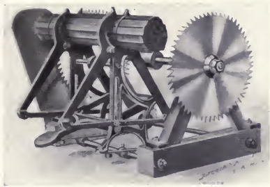
Fig. 51. Combination Lath-Binder and T-trimmer. With this machine the operator can trim the bundles of lath, simply by tilting the packing frame over from him causing the bundles to pass between the saws, thereby trimming both ends at one movement.
