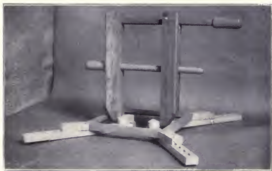
Fig. 254. Picture-Frame-Clamp.
