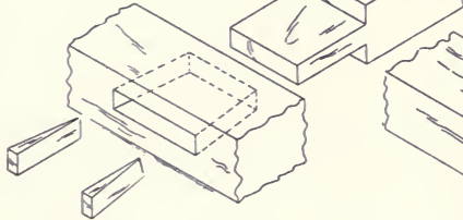
34 Wedged mortise-and-tenon
