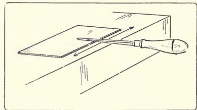
Fig. 157. Resharpening a Cabinet-Scraper: Flattening the Edge.
