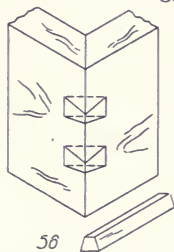
Slip-dovetail miter
