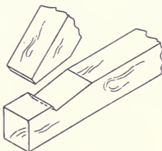
64 Oblique thrust
