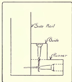
Fig. 295. Drawer Mechanism.
