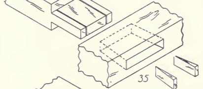
35 Wedged mortise-and-tenon
