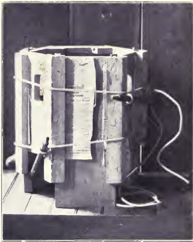
Fig. 257. One Method of Gluing up a Six-Sided Taboret.
