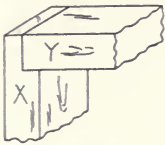
24 Rabbet
