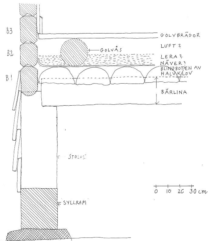
Snitt 2-2 Illustration: Kristina Linscott.
