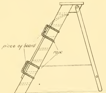
VIEW SHOWING METHOD OF BENDING AND HOLDING RUNNERS WITH BOARDS AND ROPE
