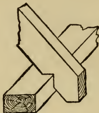
Fig. 367.—Another Type of Birdsmouth Joint.
