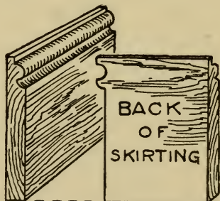
Fig. 369.—Scribing Joint on Skirting Board.
