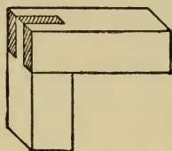
Fig. 78.—Bridle Joint.
