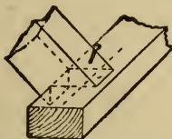
Fig. 366.—Birdsmouth Joint.
