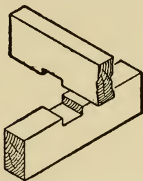
Fig. 358-9.—Notched Joint.
