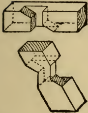
Fig. 55.—Carpentry Tie Joint.
