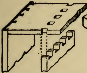
Fig. 149.—Pinning.
