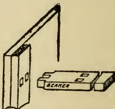
Fig. 148.—Twin Tenons.
