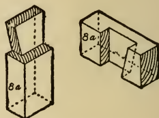
Fig. 37.—Halved Joint with One Side Dovetailed.
