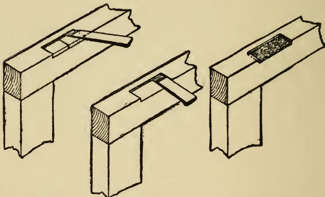
Fig. 228. Paring.
