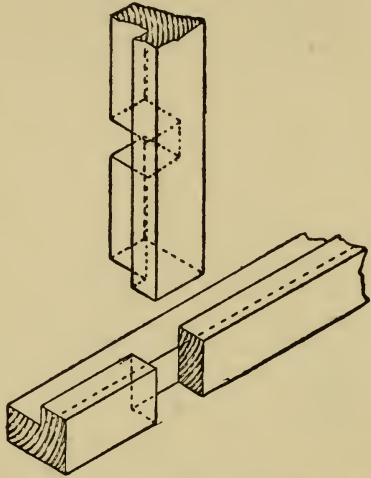
Fig. 61C.—The Halved Joints of an Oxford Frame.
