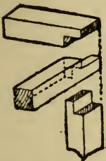
Fig. 57.—Cross Rail and Upright Halved Joint.
