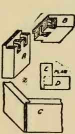
Fig. 299.— Dovetails for Small Boxes.
