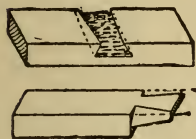
Fig. 48.—Bevelled Dovetail Half- lapped Joint.
