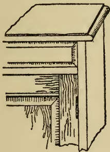
Fig. 242.—Inside Hinging.
