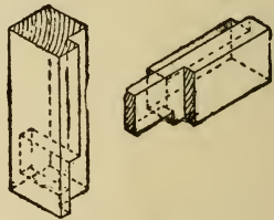
Fig. 142.—Long and Short Shouldered Tenon Joint.
