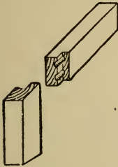
Fig. 206.—Frame Dowelling.
