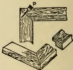
Fig. 350.—Pelleting.
