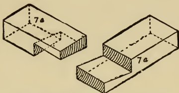
Fig. 36.—Halved Joint with Double Dovetail.
