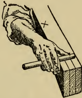
Fig. 82.—Gauging the Timber with Mortise Gauge.
