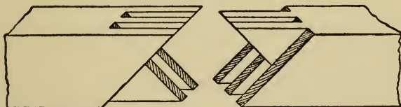
Fig. 385.—Useful Manual Training Exercise Joint.
