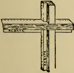
Fig. 61B.—Back View of Corner of Oxford Frame.
