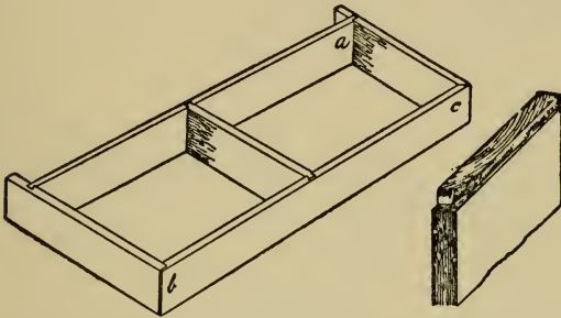
Fig. 292.—Dovetail Joints in Framing.
