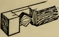
Fig. 183.—Mortise with Side Removed.
