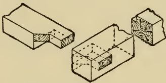
Fig. 141.—Haunched Tenon for Skylight or for Garden Frame.
