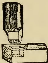
Fig. 147.—Mitred and Moulded Joint.
