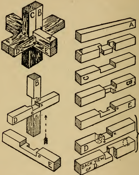
Fig. 427.—Six-piece Joint Puzzle.
