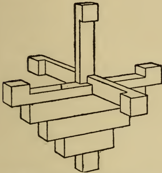
Fig. 416.—Beginning to place on the Cross Pieces.
