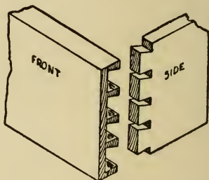
Fig. 274.—Lap-Dovetailing.
