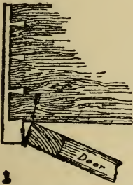
Fig. 223.—Stop-bound Door.
