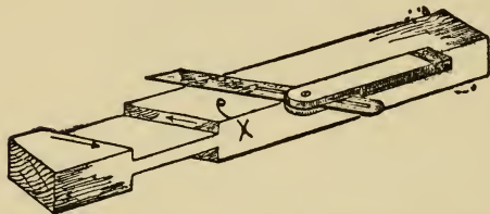
Fig. 91.—Bridle Joint at Angle other than Right Angle.
