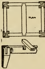
Fig. 300.— Dovetailed Footstool.
