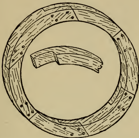
Fig. 337.—Circular Rim in Halved Segments.
