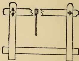
Fig. 61A.—Oxford Frame Halved Joints.
