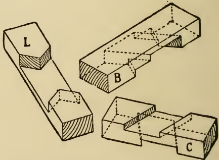
Fig. 47.—Detail of Halved Joints as in Fig. 46.
