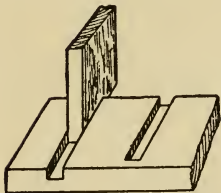
Fig. 377.—Housing Joint.
