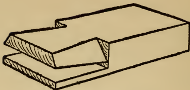
Sketch of Dovetail Piece.
