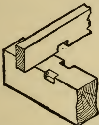
Fig. 361.—Cogged Joint.
