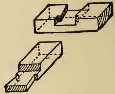
Fig. 45.—Dovetailed Halved Joint with Shoulders.
