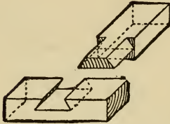
Fig. 44.—Dovetailed and Halved Joint.
