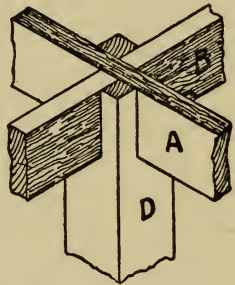
Fig. 382.—Cross-Framing Joint.
