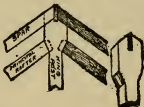
Fig. 159.—Rafter Joint.
