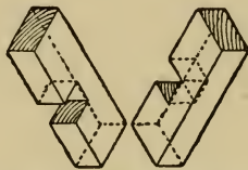
Fig. 40.—Cross Halving Joint. Fig. 41.—Cross Halving Joint, edgeways.
