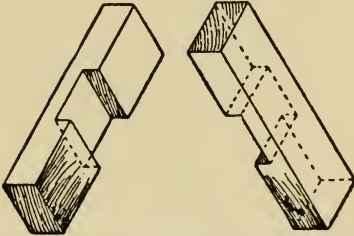
Fig. 62.—The Two Pieces of a Halved Joint.
