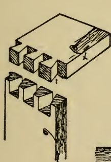
Fig. 324 —Through Dovetailing.
