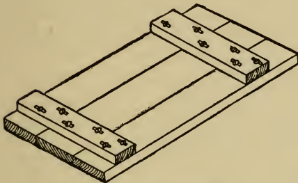
Fig. 380.—Battening.
