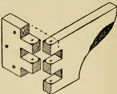
Fig. 250.—Finger Joint.
