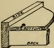
Fig. 381.—Drawer Bottom Joint.
