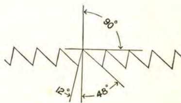
CROSS-CUT TEETH \frac{1}{4} " PITCH.
