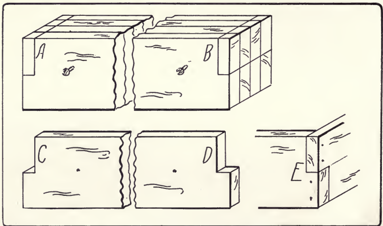
Fig. 38. Method of making and joining frame of waste-basket.
