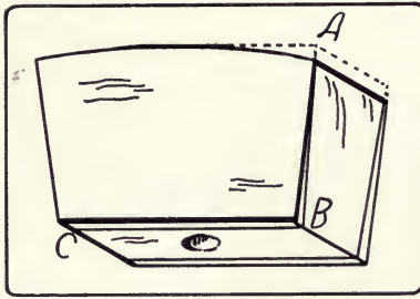
Fig. 161. Lay-out for beveled sides. (Seen from below.)
