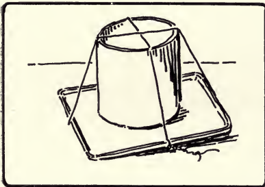
Fig. 112. Socket and pan wired together for soldering.
