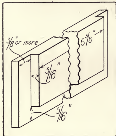
Fig. 187. Rabbetted side of box.
