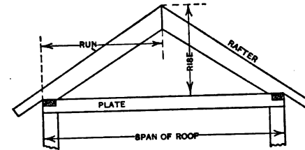
FIG. 39.—Roof Terms.
