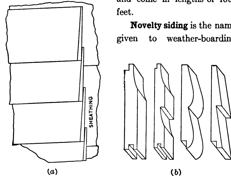
Beveled Siding or Clapboards.
