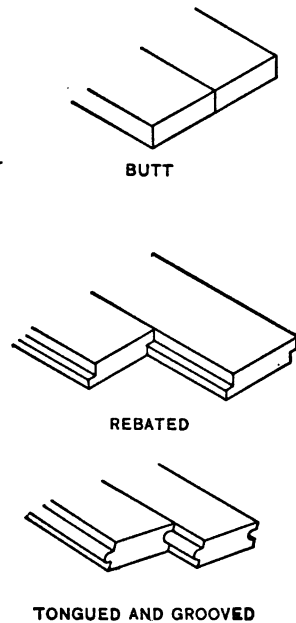
FIG. 49.—Flooring.
