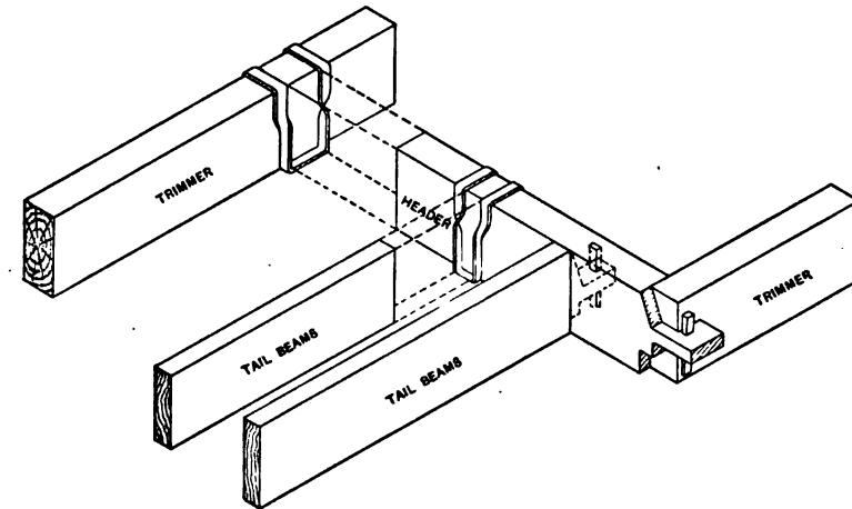
FIG. 33.—Framing Openings.
