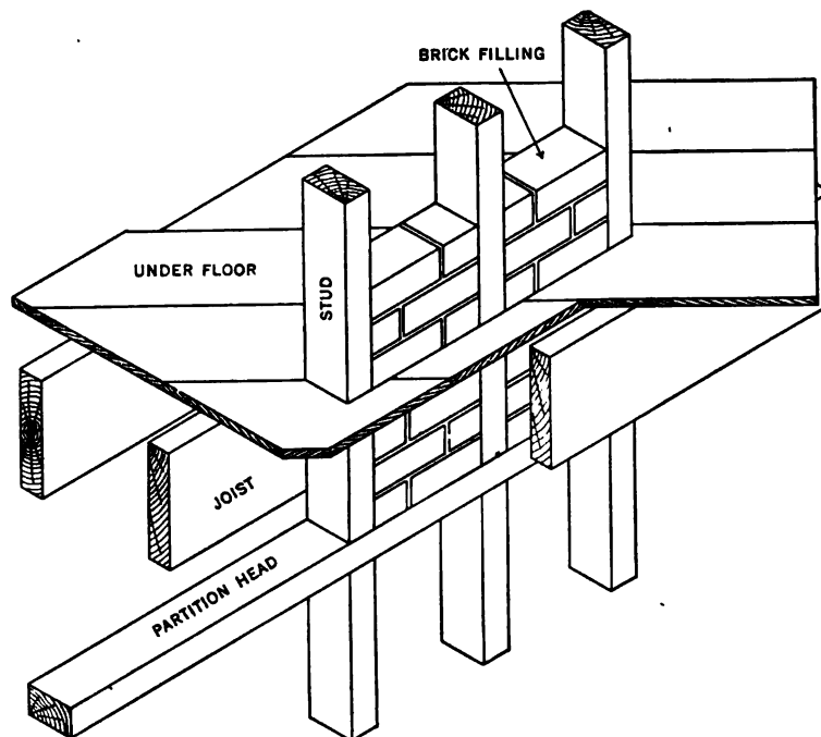
FIG. 35.—Bearing Partition.
