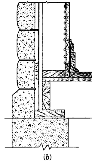
(b) Cement Block Veneer.
