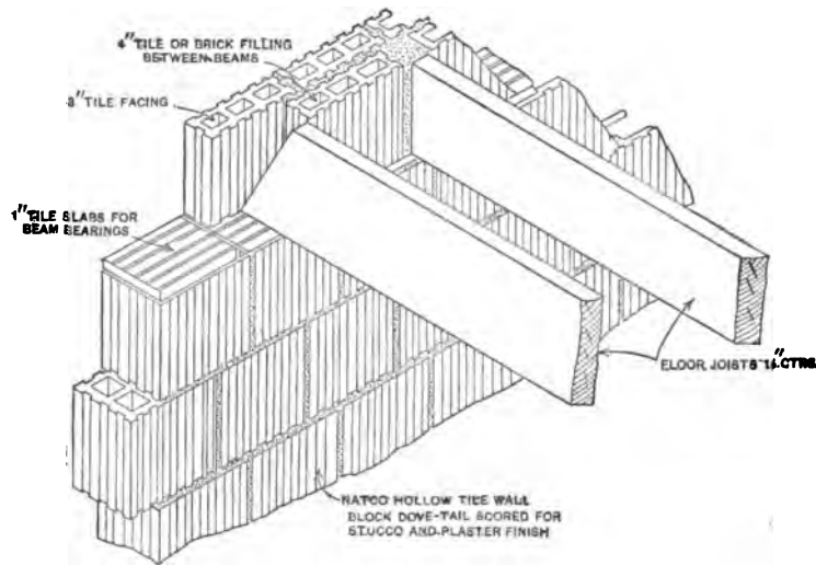
FIG. 28.—Detail of Wall and Floor Construction for Hollow Tile Walls with Wood Floors.
