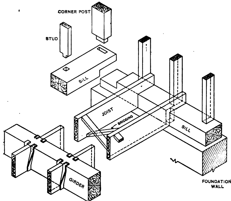
FIG. 32.—Framing Details.
