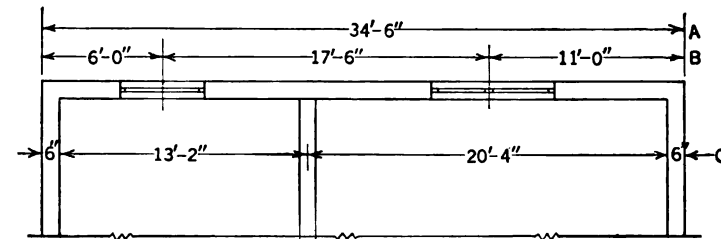
FIG. 7.—Dimensioning.
