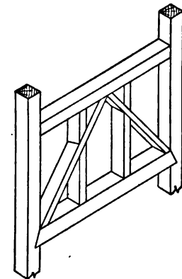
FIG. 34. Truss Over an Opening.
