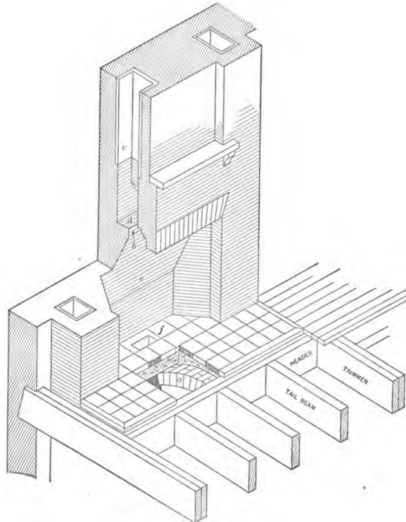
FIG. 37.—Construction of Chimney and Fireplace.
