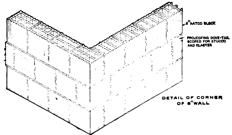
FIG. 27.—Detail of Corner of 8" Hollow Tile Wall.
