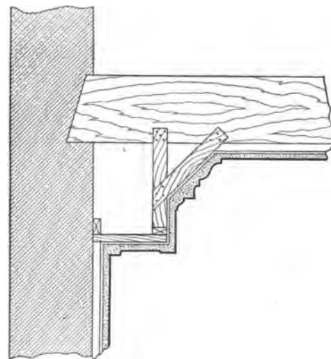
FIG. 47.—Furring for False Beam.
