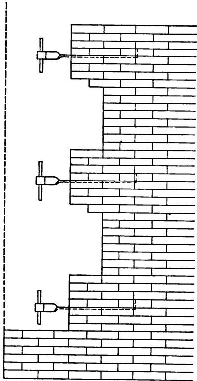
FIG. 21.—Brick Wall with Toothings and Iron Anchors.
