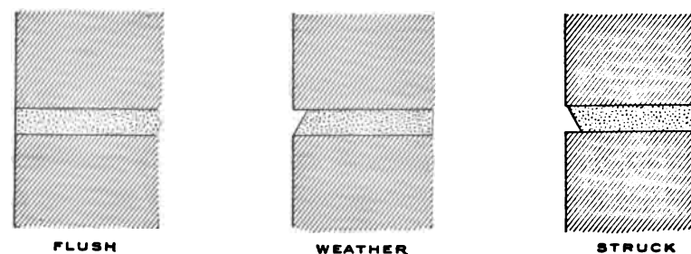
FIG. 12.—Brick Masonry Joints.
