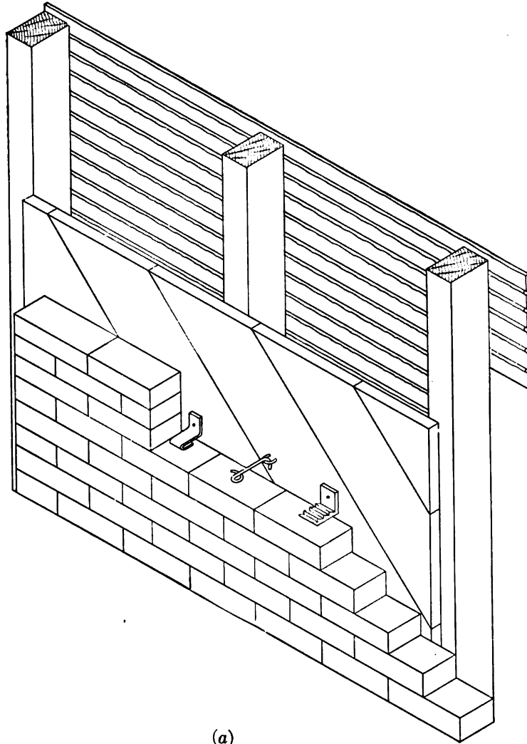
(a) Brick Veneer.
